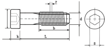
Hexagon socket head cap screws with low head
