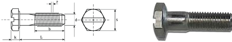
Hexagon slotted head bolts - Metric pitch thread
