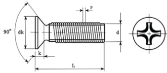
Flat head phillips countersunk screws
