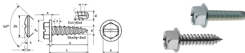
Hexagon washer head with one slot tapping screws
