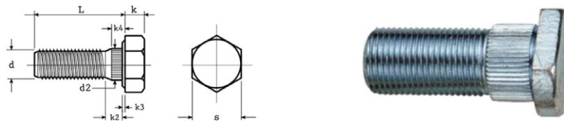
Hex knurling bolts
