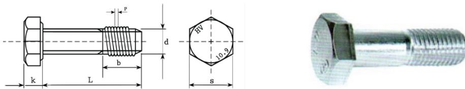
High strength structural bolt (HV)
