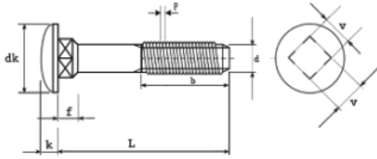
Mushroom head square neck (cap square neck bolts)
