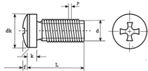
Cheese head phillips screws
