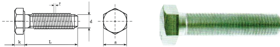
Hexagon head bolts - Metric pitch thread
