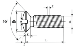
Slotted raised countersunk head screws
