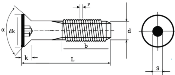
Hexagon socket countersunk head screws
