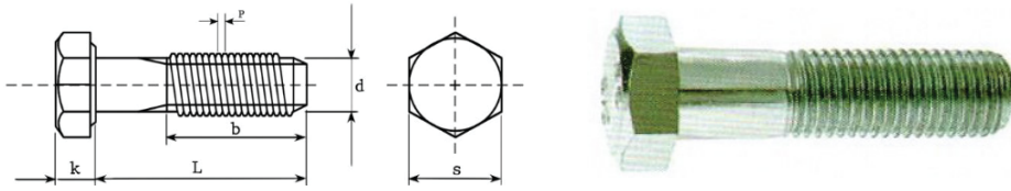
Hexagon head bolts - Metric pitch thread
