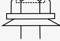
HEX WASHER HEAD WITH BOUNDED WASHER
